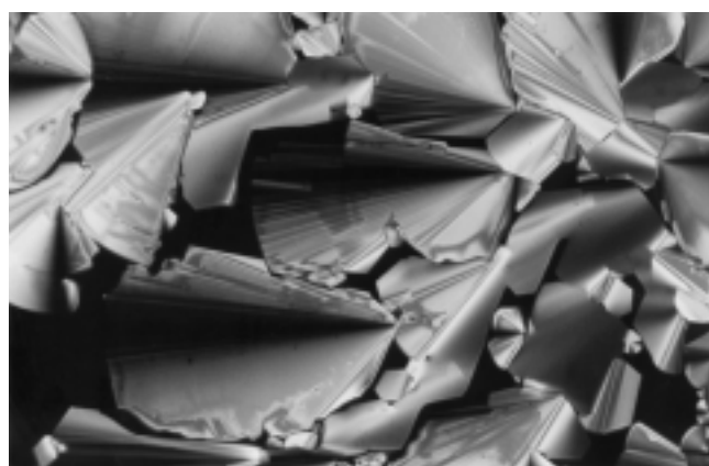
Figure 1. Optical texture of A as it appears when viewed through cross-polarizing filters at 240 °C (×100).
